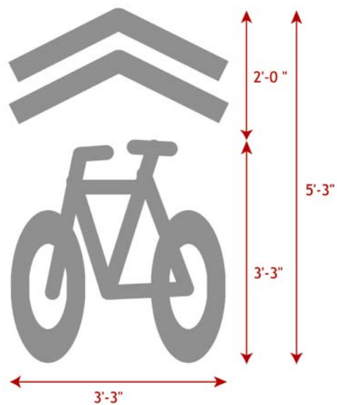
Bike-and-chevron marking
